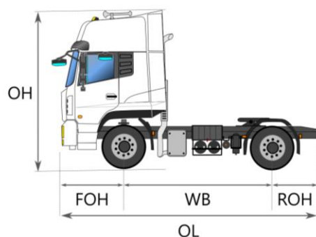
Chassis Dimension (mm)
