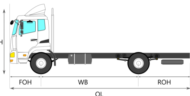
Chassis Dimension (mm)
